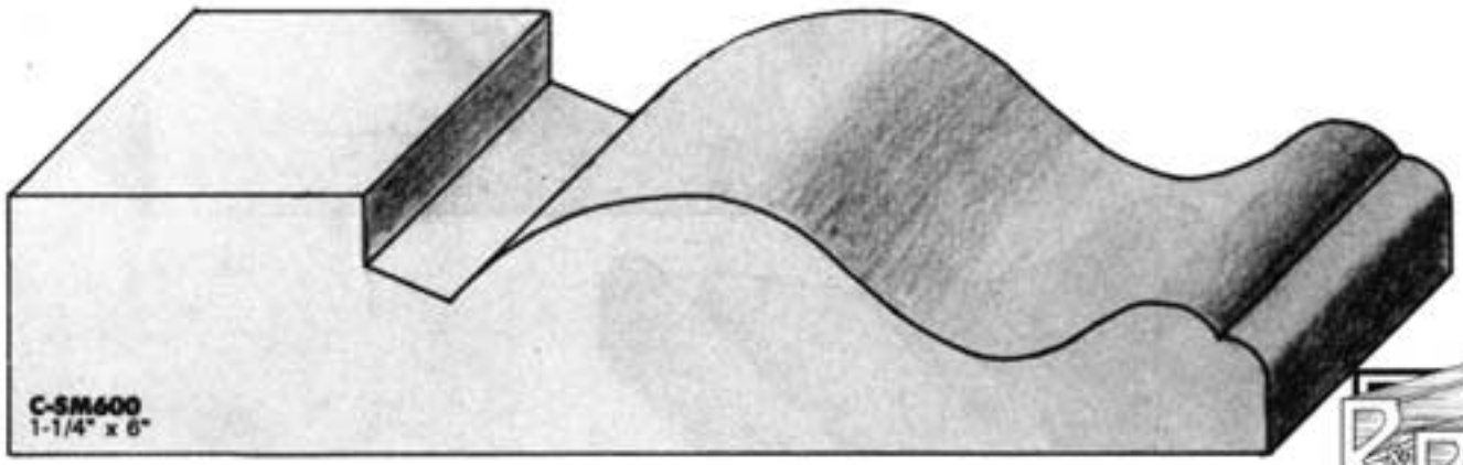
C-PA550 13/16" x 5-1/2"
