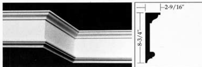
No. 37004 Covington
